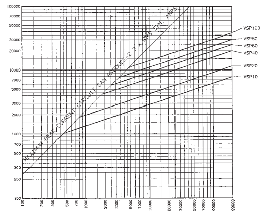
Peak Let-Thru Current Data
