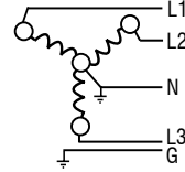
3 Phase Wye 4 Wire + Ground
