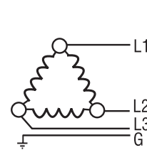
3 Phase Delta 3 Wire + Ground
