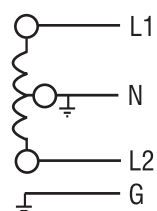
Split Phase 3 Wire + Ground
