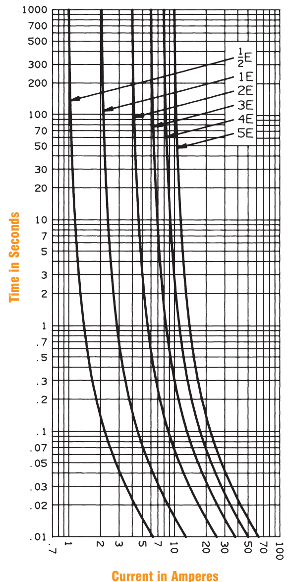
Melting Time – Current Data - PT Fuses - 4800V
