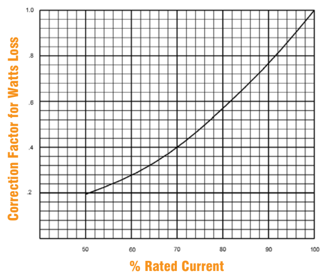
Watts Loss vs % Rated Current
