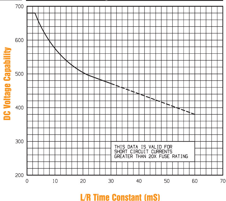
DC Voltage vs. Time Constant
