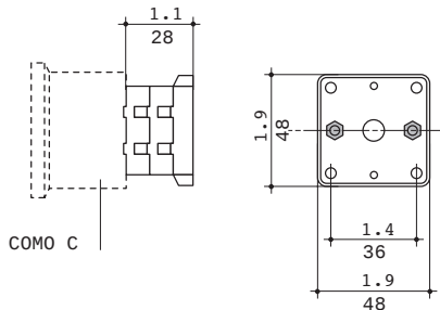
Two aux.contacts
