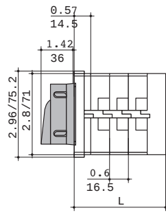
Door mounted with direct operation
