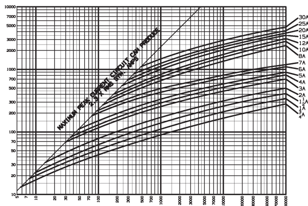
Peak Let-Thru Current Data
