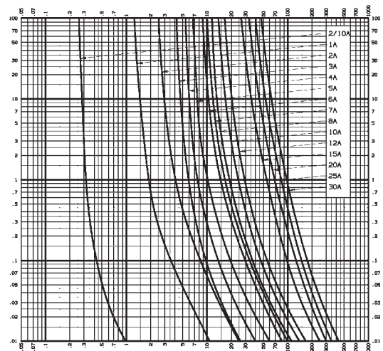
Melting Time – Current Data
