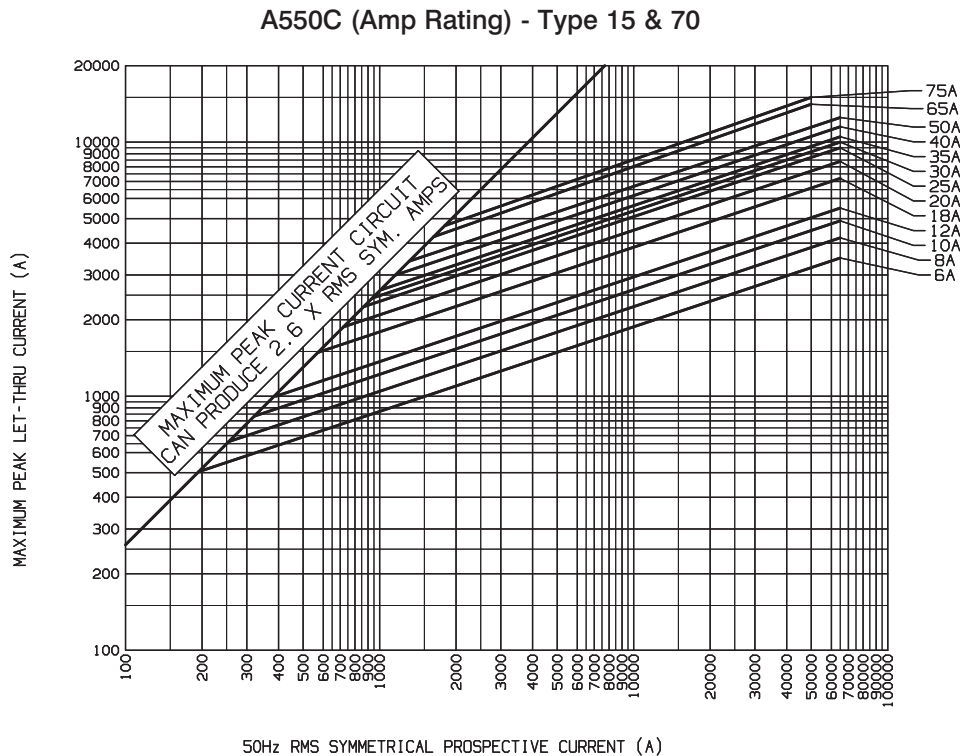
Peak Let-Thru Current Data 5.5kV Type 15 & 70
