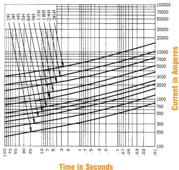
Minimum Melting Time – Current Data, 4.8kV Fuses
