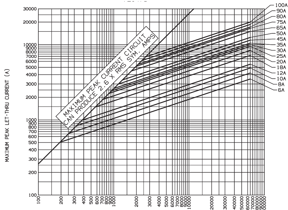
Peak Let-Thru Current Data 4.3kV Type 15 & 70
