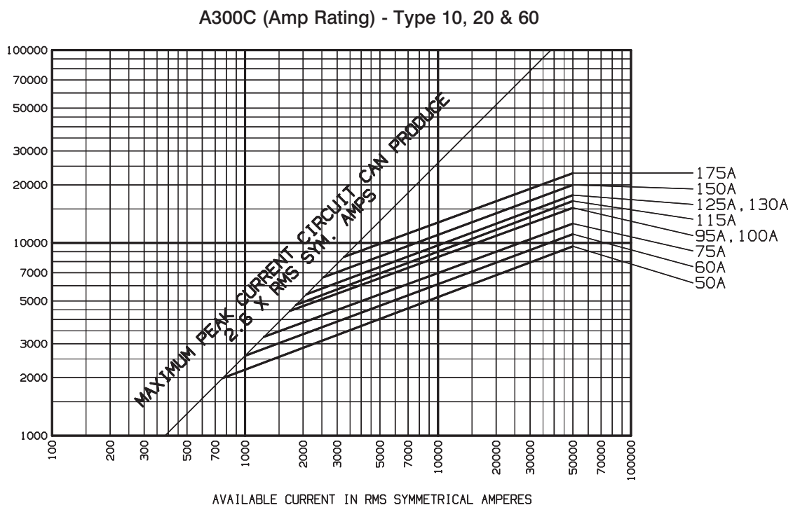
Peak Let-Thru Current Data 3.0kV Type 10, 20 & 60
