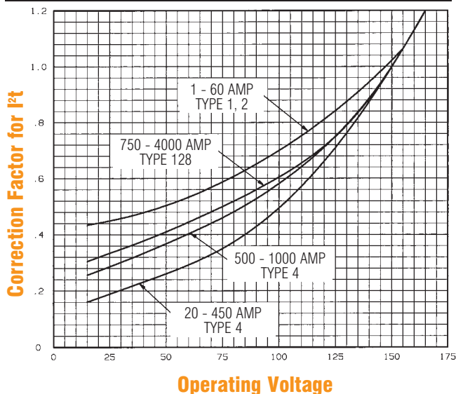
Clearing I 2 t vs Working Voltage
