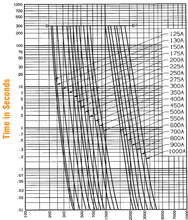
Melt Time - Current Data A15QS 125 to 1000
