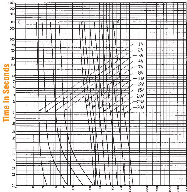
Melt Time - Current Data A15QS 1 to 30
