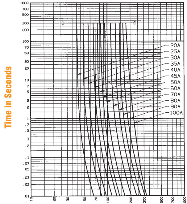
Melt Time - Current Data A15QS 20 to 100
