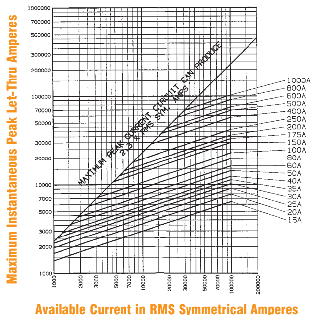
Peak Let-Thru Data – A150X15 to 1000, 1500 VAC
