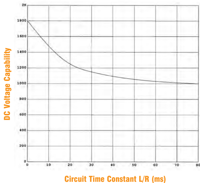
DC VOLTAGE CAPACITY VS. TIME CONSTANT
