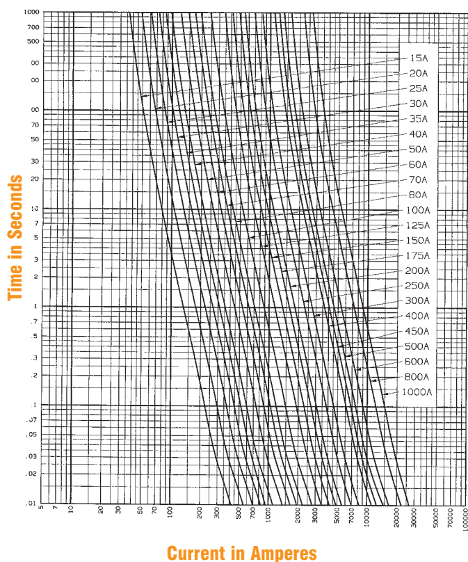
Melting Time – Current Data, 1500V Fuses
