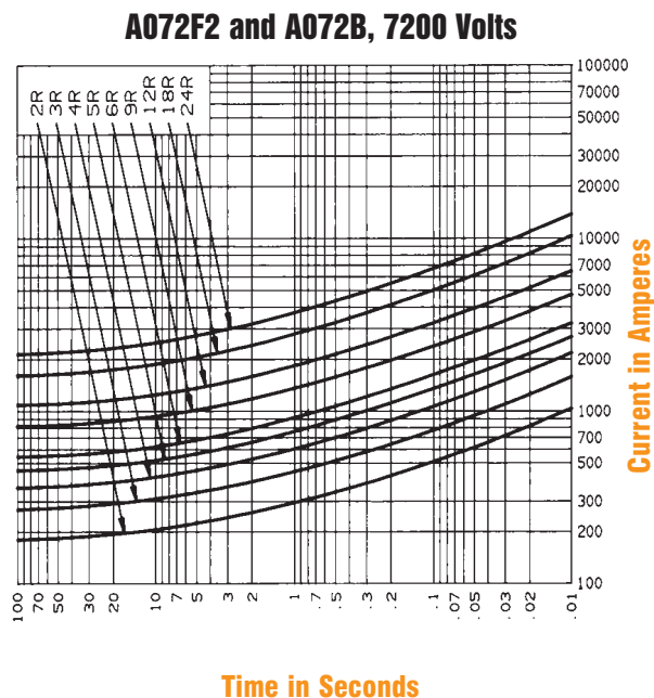
Minimum Melting Time – Current Data, 7.2kV Fuses
