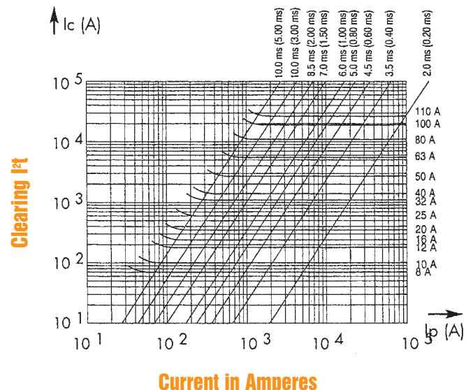
Total Clearing I^2t
