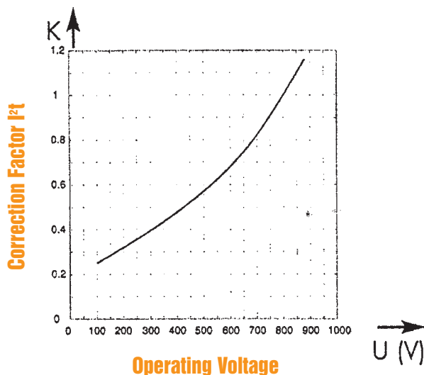
Clearing I^2t vs. Operating Voltage
