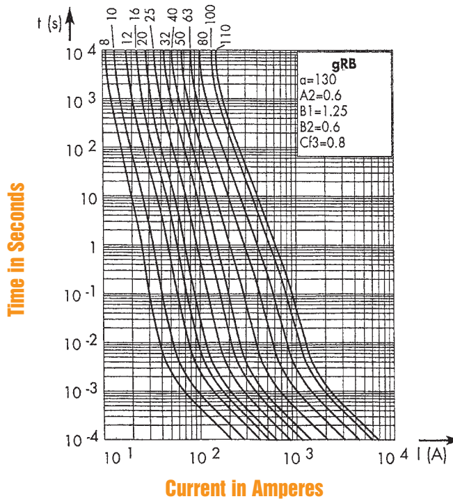
Melting Time Current Data
