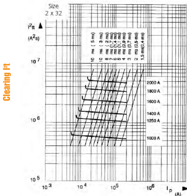
Clearing I²t Data 2X32
