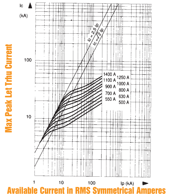
Peak Let-Thru Current Data
