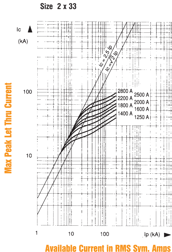
Peak let-thru Data 2X33
