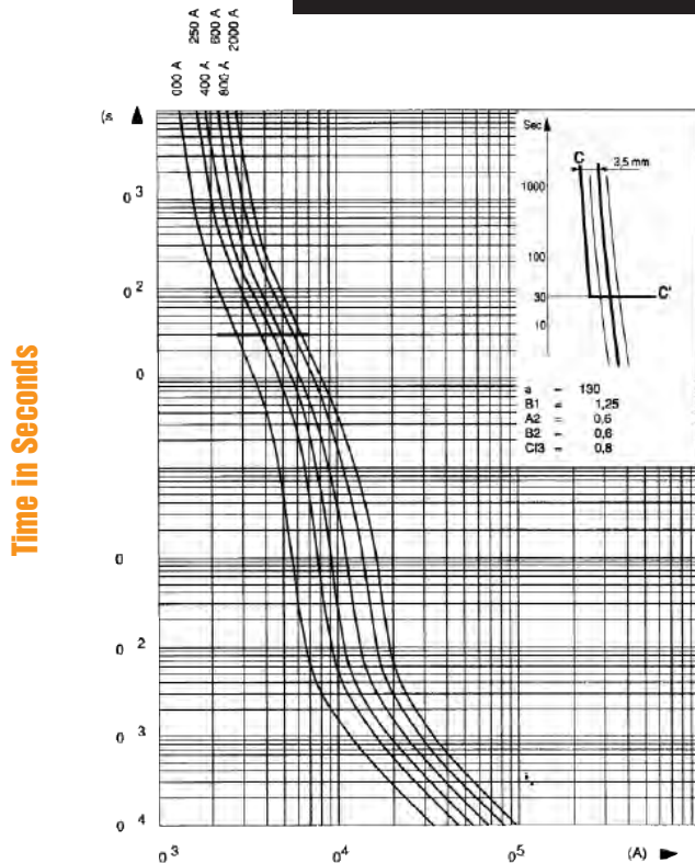
Melting Time Current Data 2X32
