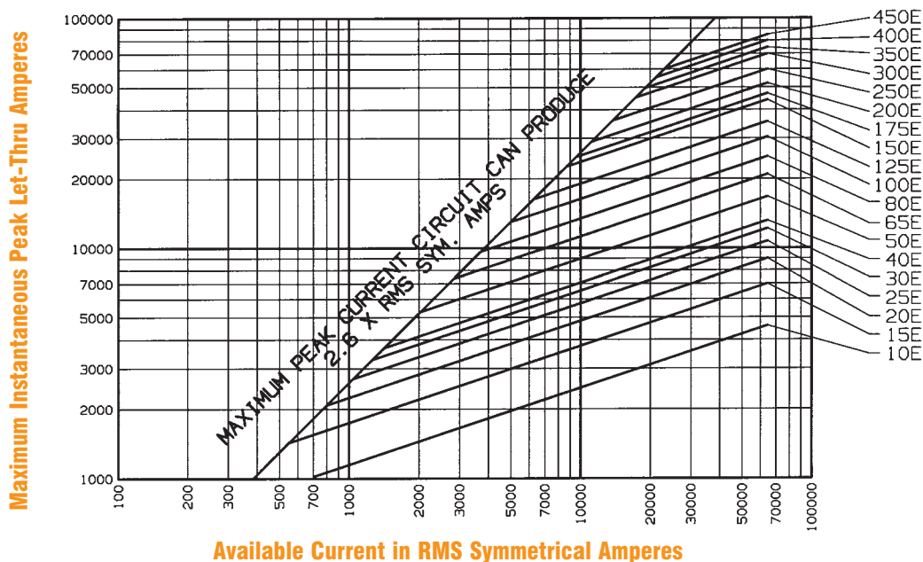
Peak Let-Thru Current Data, E-Rated Fuses
