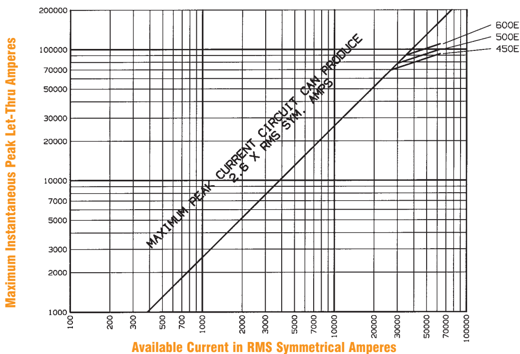
Peak Let-Thru Current Data, E-Rated Fuses
