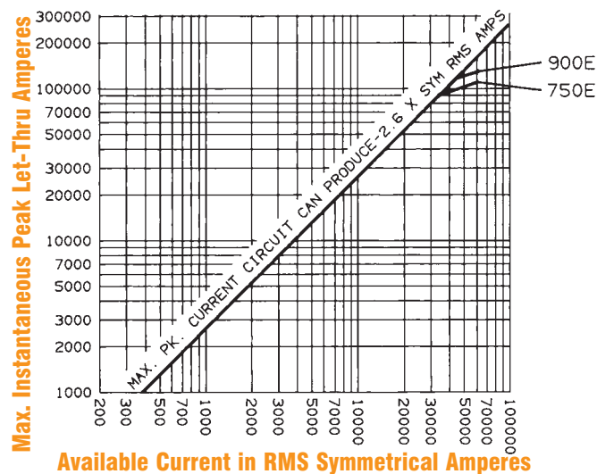
Peak Let-Thru Current Data – 5.5kV Bolt-in Fuses
