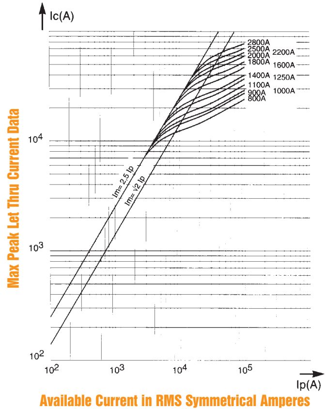
Peak let thru Current Data
